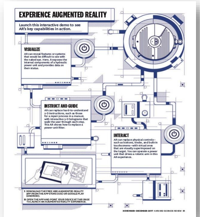
[Marker Based]
